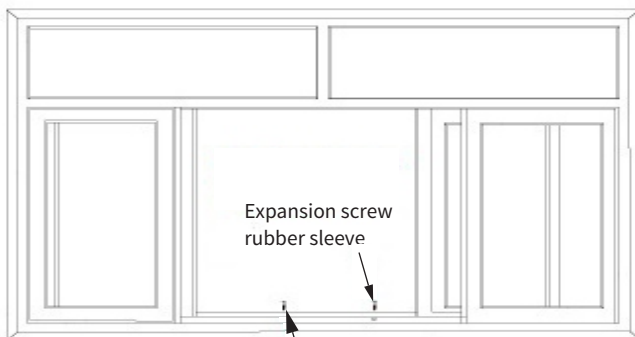
Base on the clip, the first drill 2 expansion screw rubber sleeves on the window sill
